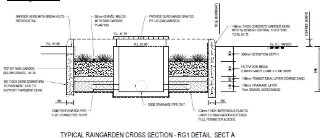
Figure 3: Raingarden Typical Cross-Section.
