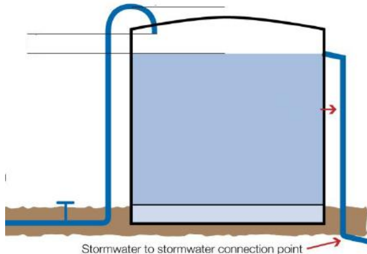
Figure 2: Typical Rainwater tank Cross-Section.
